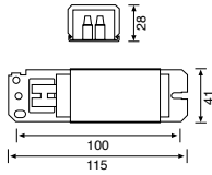
JK026 26W Mekanik Balast 2,00 USD 40 Ad. 100x41x28
